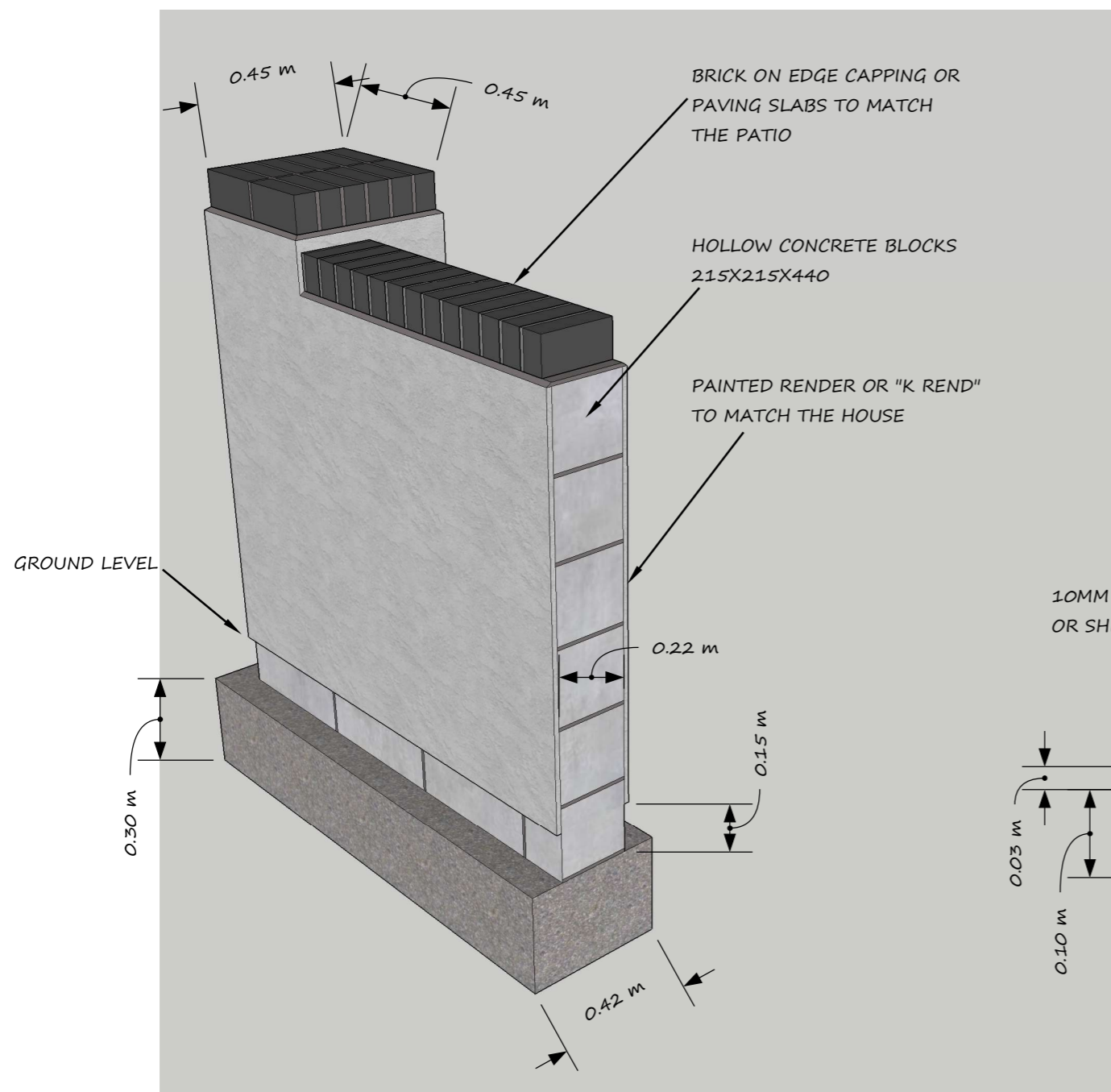
CROSS SECTION OF FRONT WALL
