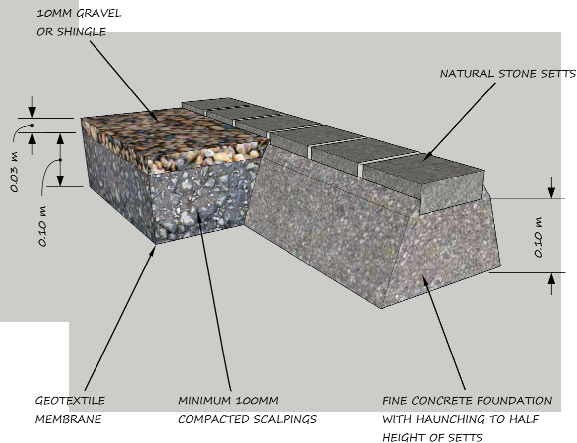
CROSS SECTION OF SETT EDGING AND DRIVE
